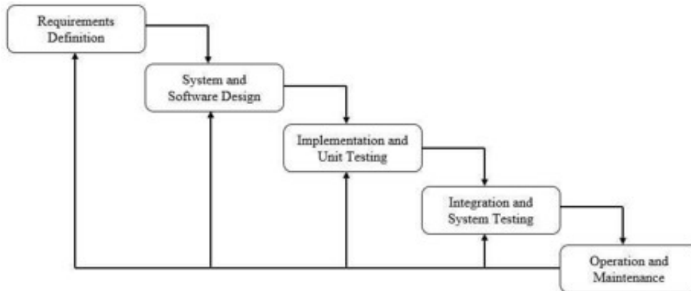
Figure 1. Metode Waterfall
