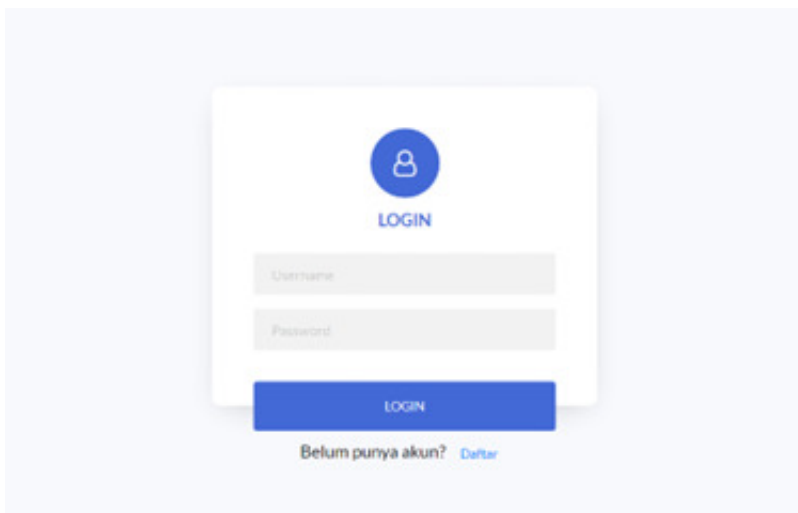
Figure 4. Halaman Login
