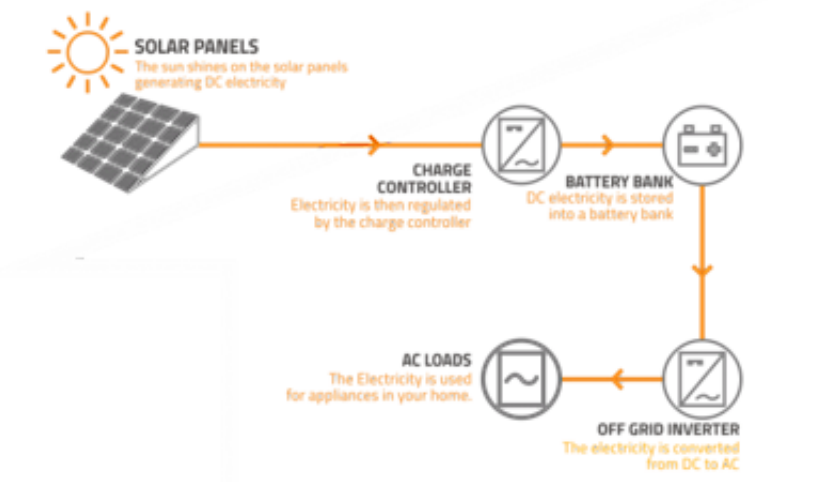
Figure 1. Pembangkit listrik tenaga surya Off-Grid
