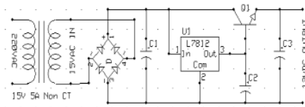
Gambar 7. Power Supply
