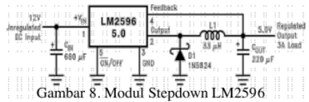
Gambar 8. Modul Stepdown LM2596
