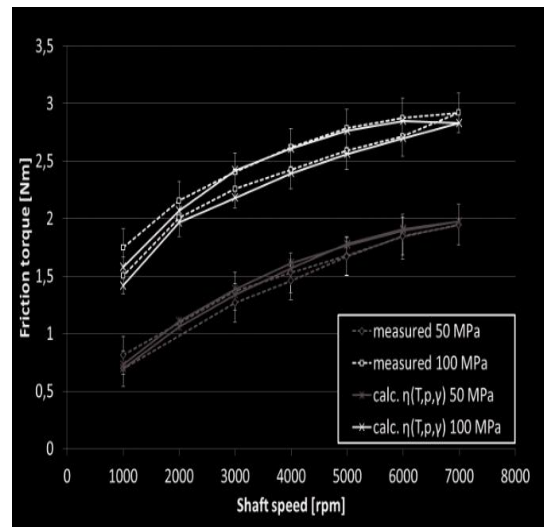
Figure 7. Comparison of Average Friction Torque Measured on the Test Rig with Average Friction Torque Simulated Using the Full Oil Model \eta(T,p,\gamma) at Specific Loads of 50 and 100 MPa
