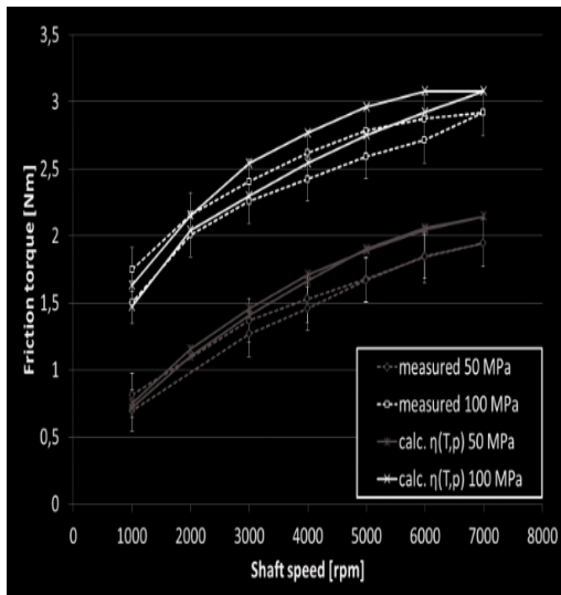
Figure 6. Comparison of Average Friction Torque Measured on the Test Rig and Average Friction Torque Simulated Using the Pressure-Dependent Oil Model \eta(T,p) at Specific Loads of 50 and 100 MPa
