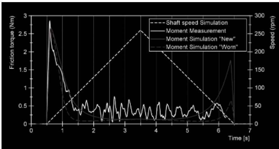
Figure 12. Comparison of Measured and Calculated Torque during a Shaft Start-Stop Cycle Using New and Worn Surface Roughness
