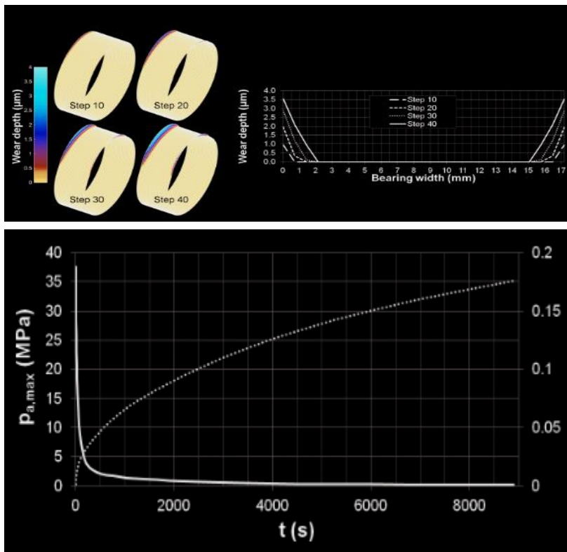
Figure 10. Surface profile on the left and a sectional view of the surface profile at the location of maximum wear depth during the iterative manufacturing process on the right.
