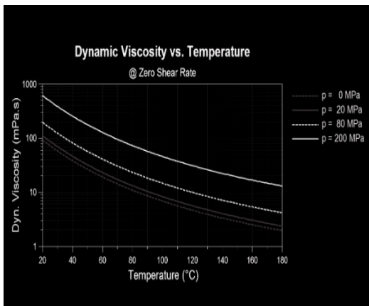
Figure 1. Temperature dependence of viscosity of lubricant oW20 at different pressures
