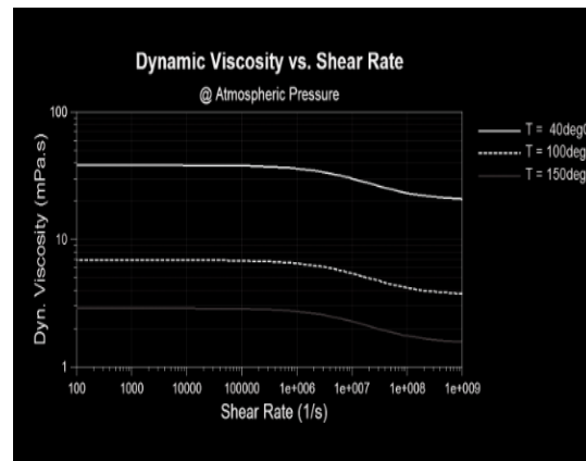
Figure 2. Shear viscosity dependence for oW20 lubricating oils at different temperatures
